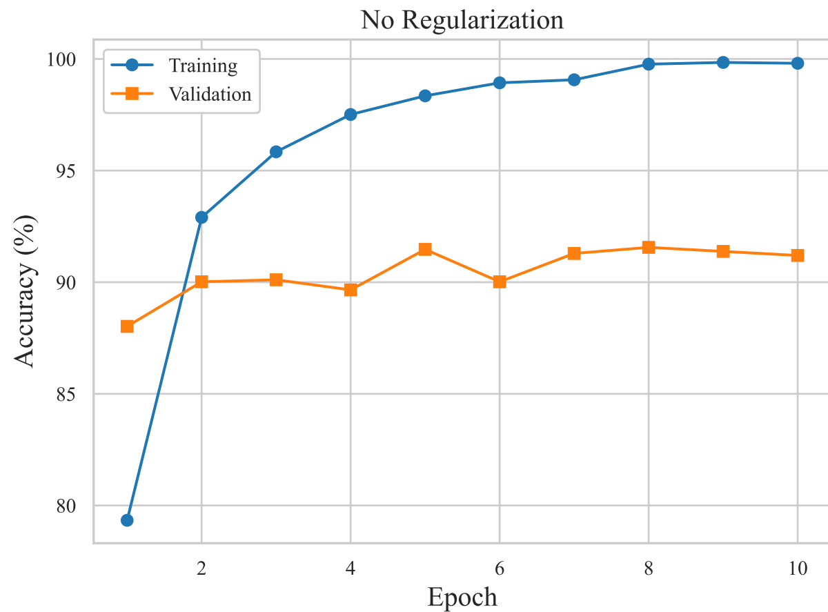
Plot 3: Training and Validation Accuracy vs. Epoch
